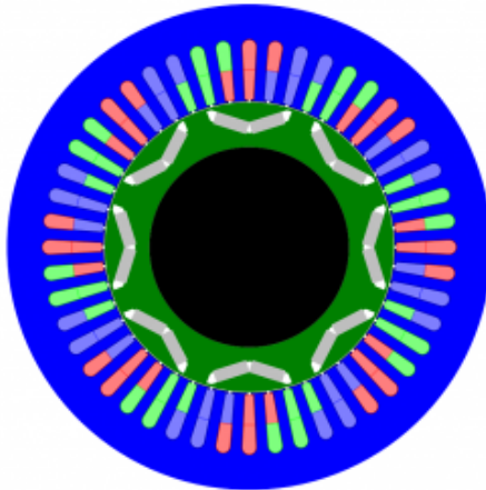
Interior Permanent Magnet Synchronous Machine (Prius 2004, automotive application)
